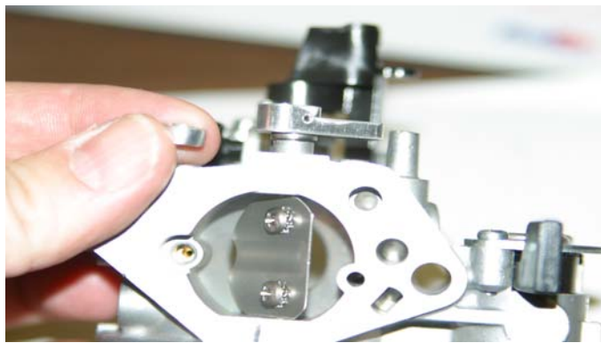
FPX Metal Type installed in Honda GX270 carburetor.
